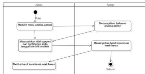
Gambar 5. Activity Diagram
