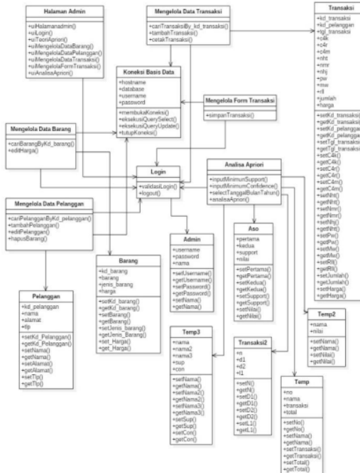
Gambar 3. Class Diagram
