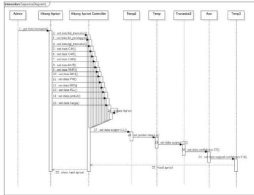
Gambar 4. Sequence Diagram
