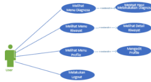
Gambar 2 Use Case Diagram User
