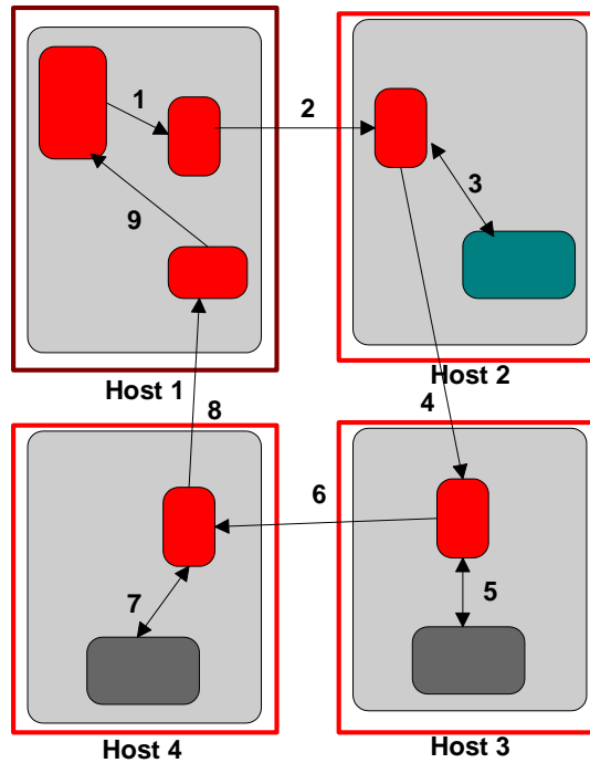
Gambar 9: Implementasi proses pencarian aglet metode itinerary
